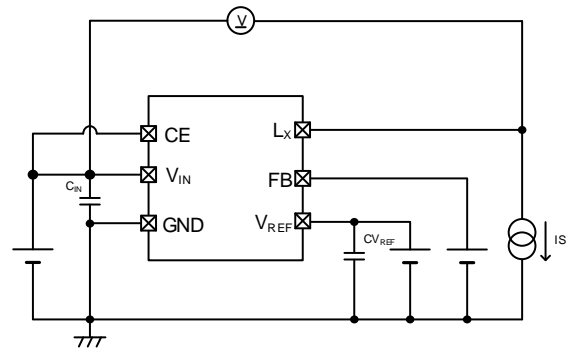
< Test Circuit No.⑥ >
