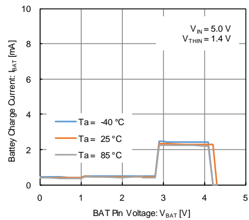
(9) Battery Charge Current vs. BAT Pin Voltage ( R_{ISET} = 59 k \Omega , Cold Operation)
