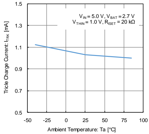
(4) Trickle Charge Current vs. Ambient Temperature
